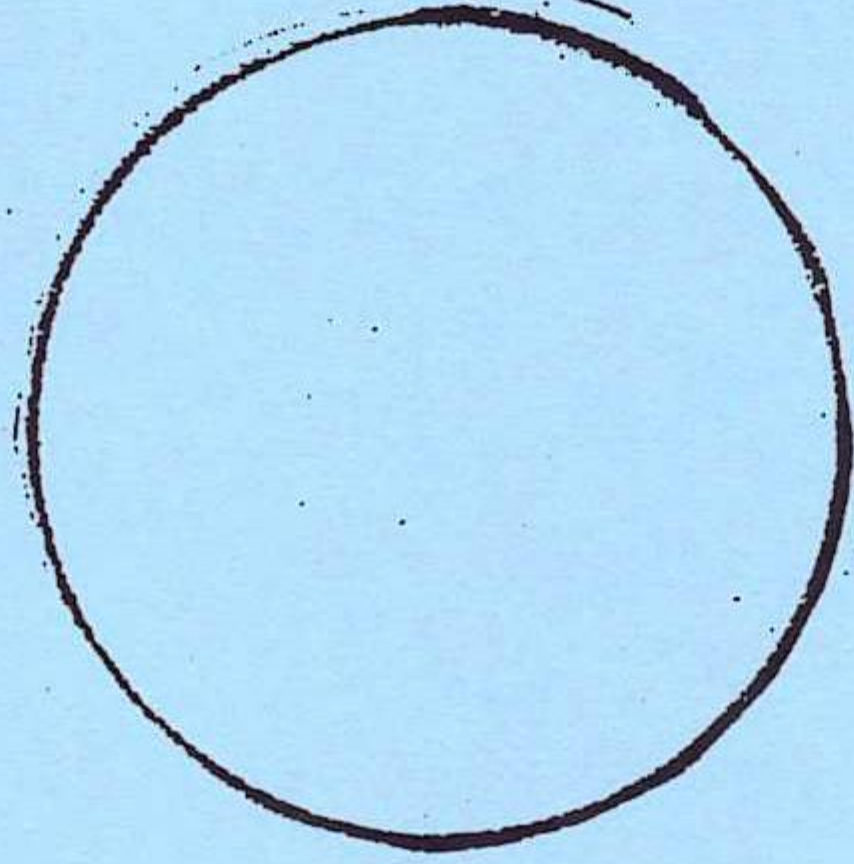
Neptune
